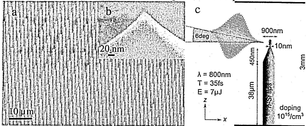
Figure 1. Images and schematic of emitter structure: (a) Scanning electron microscope (SEM) image of uniform array of high-aspect-ratio Si columns with 5 \mu\text{m} pitch. (b) SEM close-up of a single tip. (c) Schematic of a single 800 nm pulse interacting with a single silicon tip. \lambda is the laser wavelength, T is the pulse duration, and E is laser energy. (Swanwick, Michael E., et al. "Nanostructured ultrafast silicon-tip optical field-emitter arrays." Nano letters 14.9 (2014): 5035-5043.)
