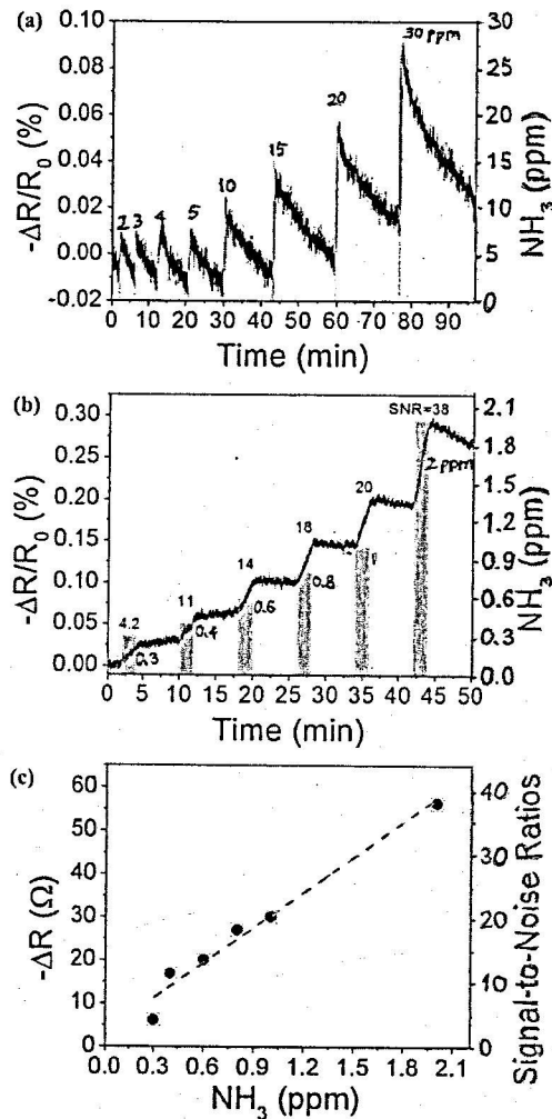
Figure 2. Sensor response plots show percentile resistance change versus time of the MoS 2 film with a bias voltage of 0.5 V, upon consequent NH 3 exposures at various concentrations: a) from 2 ppm to 30 ppm and b) 300 ppb to 2 ppm. The gray vertical bars indicate NH 3 gas injections for: a) 15 s and b) 2 min, respectively. The signal-to-noise ratio (SNR) of each folding curve is shown to verify a sensible signal. c) Plots of resistance change (black solid circles) and signal-to-noise ratios (gray open boxes) as a function of NH 3 concentration. The linear dashed line indicates the fitted line. (Source: Lee, Kangho, et al. "High-performance sensors based on molybdenum disulfide thin films." Advanced materials (Deerfield Beach, Fla.) 25.46 (2013): 6699-6702.)
